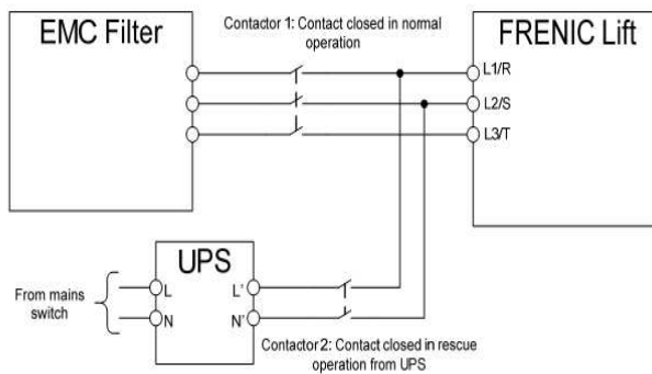
Connection of UPS for rescue operation (example)
